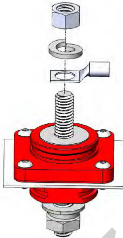
Figure 7.0 – Lug Placement on PHI Battery Threaded Stud
