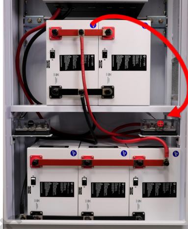
Figure 8.0 - PHI Battery Wiring Using Interconnecting Busbars
